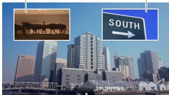
Background video
