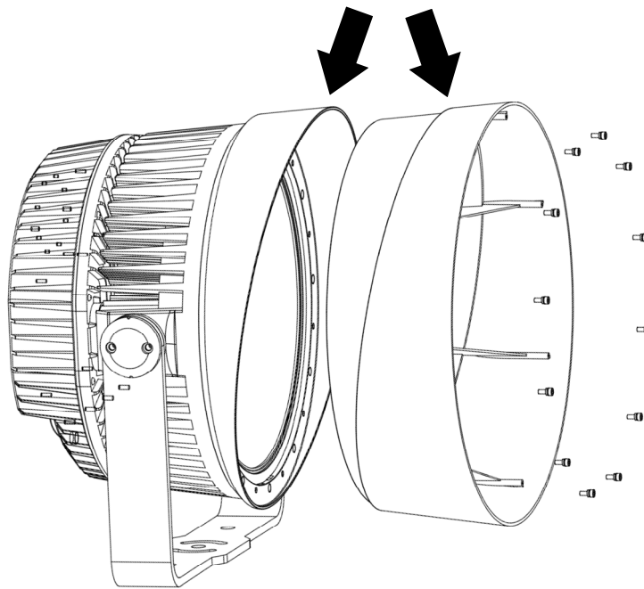
Figure 6. Snoot installation
