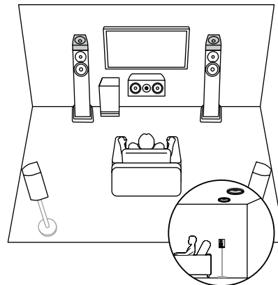
5.1.4 ch (Dolby Enabled Speakers (Front) and Top Rear) (→p36)
