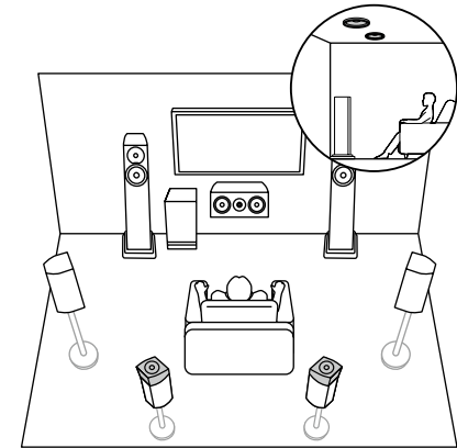
7.1.4 ch (Top Front and Dolby Enabled Speakers (Surround Back)) ( → p37 )
