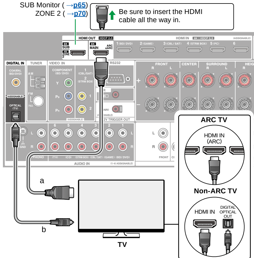
a HDMI cable, b Digital optical cable
