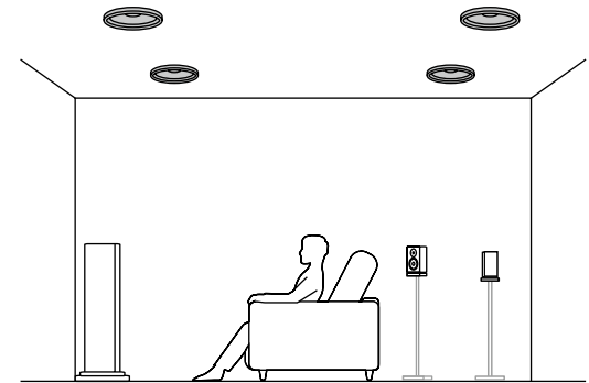
7.1.4 ch (Top Front and Top Rear) (→p37)
