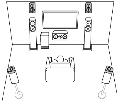
5.1.4 ch (Front High and Dolby Enabled Speakers (Surround)) (→ p36 )
