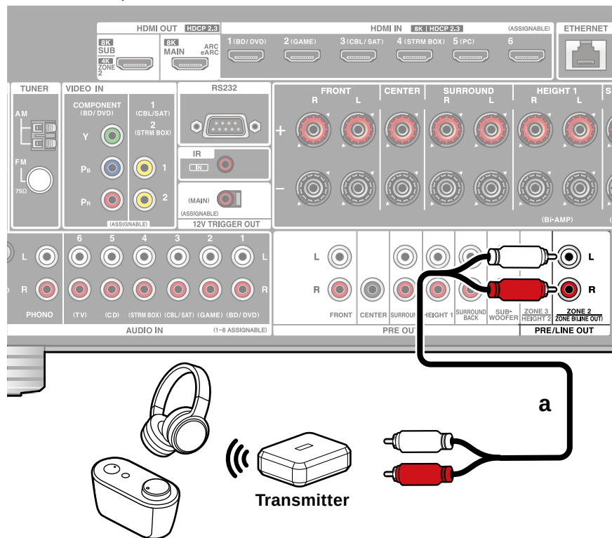
a Analog audio cable
