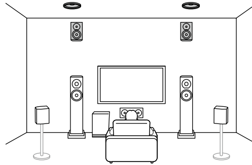
5.1.4 ch (Front High and Top Middle) (→ p36 )
