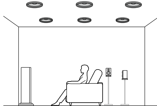
7.1.2 ch (Top Front or Top Middle or Top Rear) (→ p35 )
