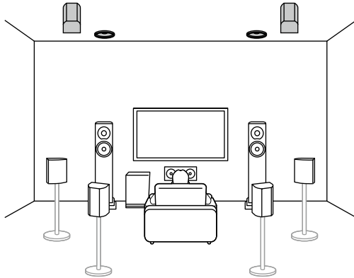
7.1.4 ch (Top Front and Rear High) ( → p37 )
