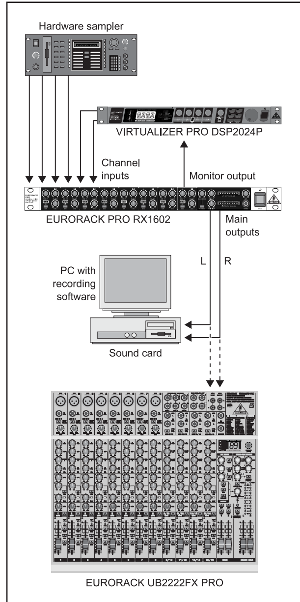
Fig. 3.2: Sampler/PC application
